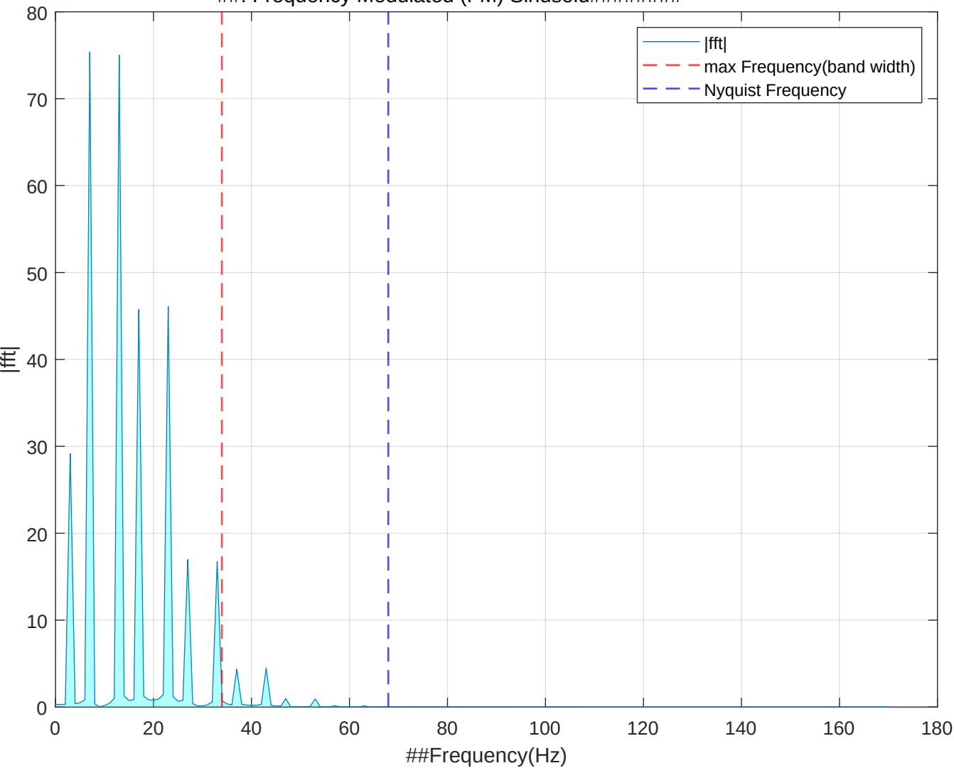
##: Frequency Modulated (FM) Sinusoid#####
